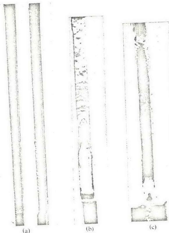
Fig. 6. Shocked powder of \text{SiO}_2 under different conditions: a - long container and large charge, size 0.5 of real size, b - short container and small charge, c - double shocked powder, band c being twice their original size.
