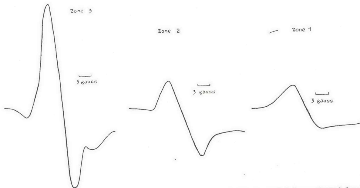
Fig. 5. EPR (electron paramagnetic resonance) spectra of the paramagnetic defect in shocked zirconium of zone 3, 2 and 1.
